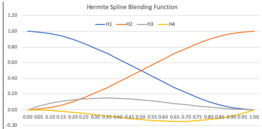
Figure 3.10: Hermite spline blending functions
