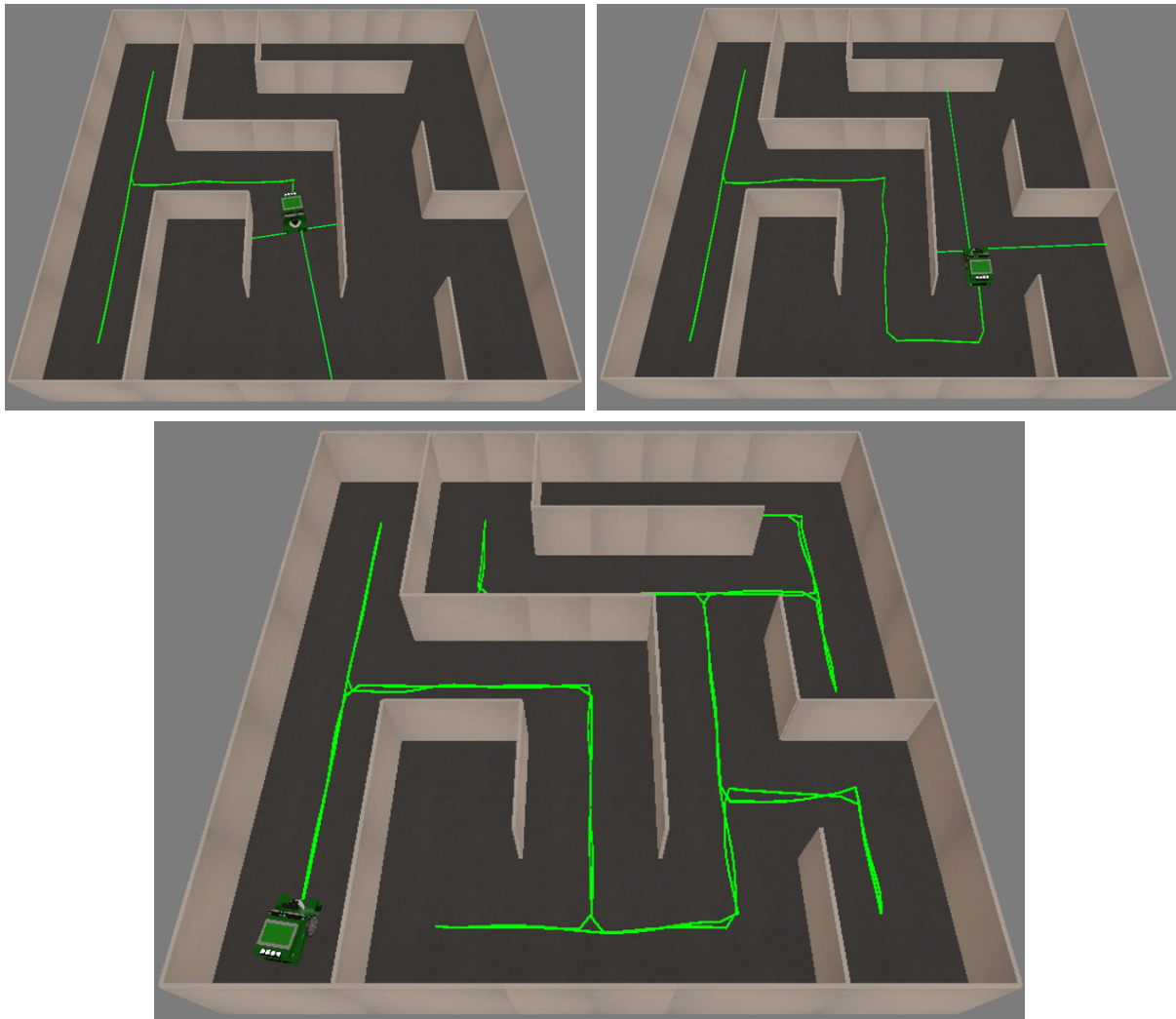
Figure 9.6: Maze-driving with P -controller for pose correction
