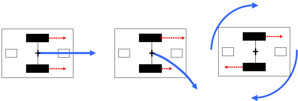
Figure 1.3: Differential drive principle
