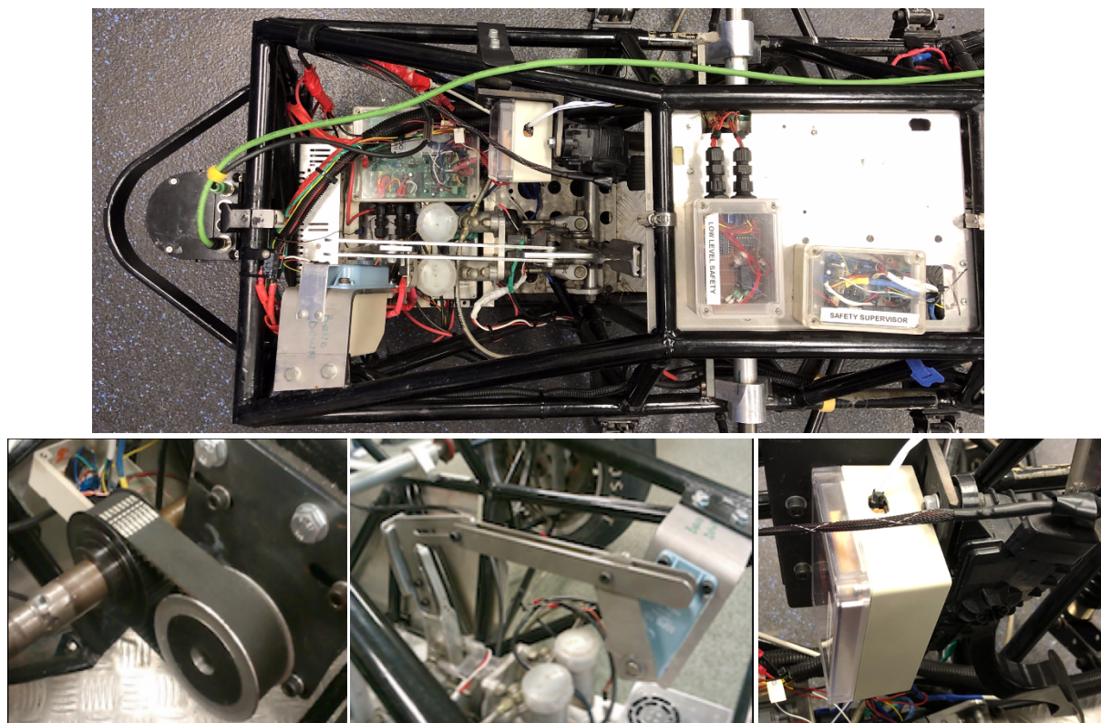
Figure 14.2: Drive-by-wire system: steer, brake, accelerate
