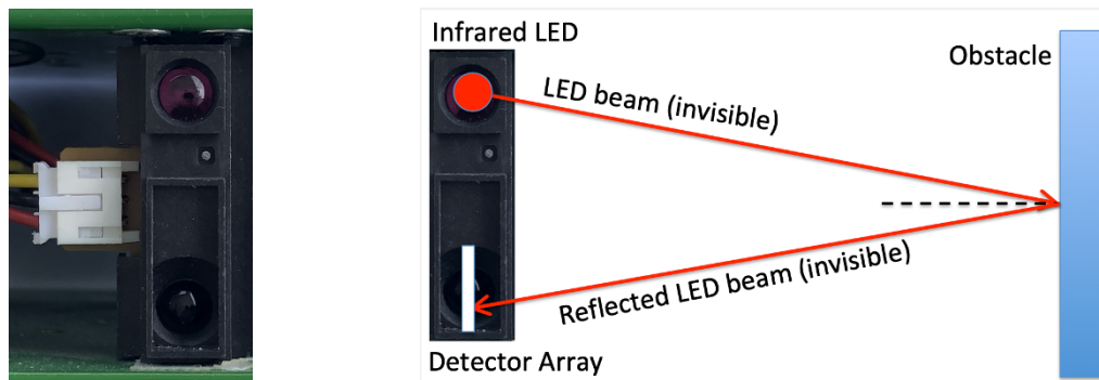
Figure 1.6: Sharp PSD sensor (left) and measurement principle (right)
