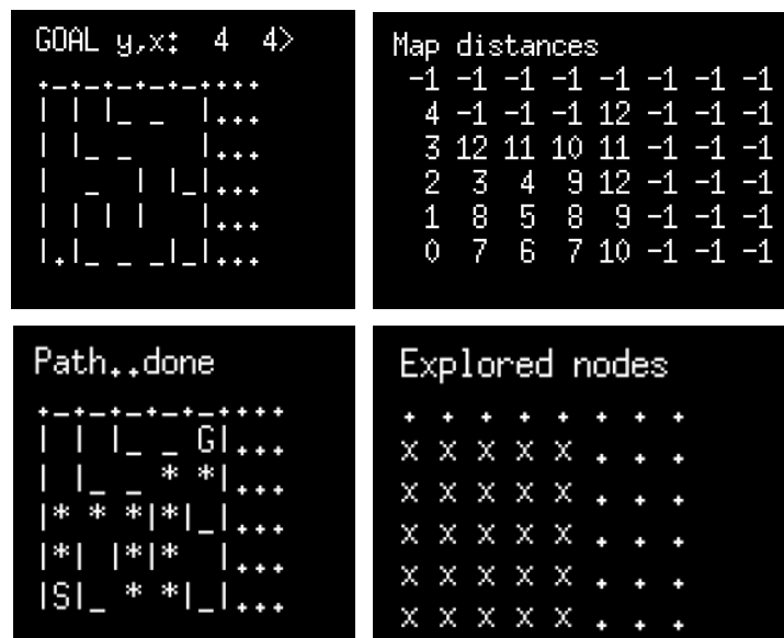
Figure 9.15: Internal representation, flood-fill, shortest path and nodes
