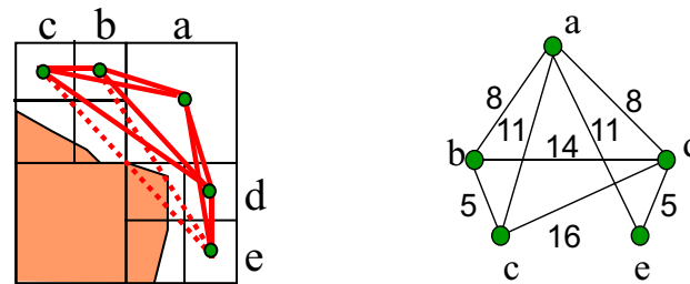
Figure 10.7: Quadtree step 4: collision paths and constructed graph
