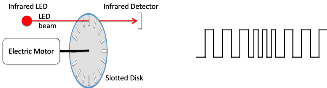
Figure 1.5: Encoder disk principle (left); encoder output signal for slow-fast-slow rotations (right)
