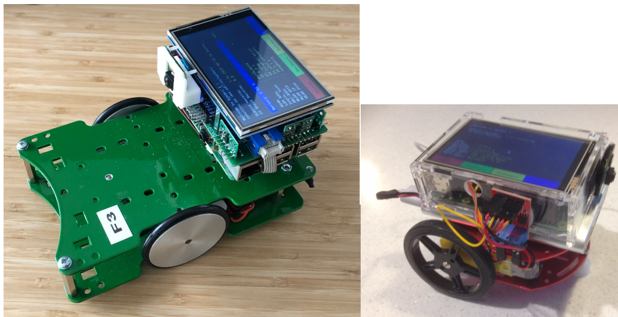
Figure 1.13: SoccerBot S4 (left), and Mule simple robot chassis (right)
