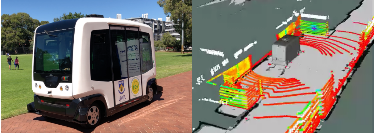
Figure 14.8: nUWay-1 shuttle bus on campus with Lidar point cloud
