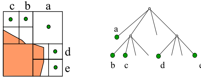
Figure 10.6: Quadtree step 3: free-space centers become nodes
