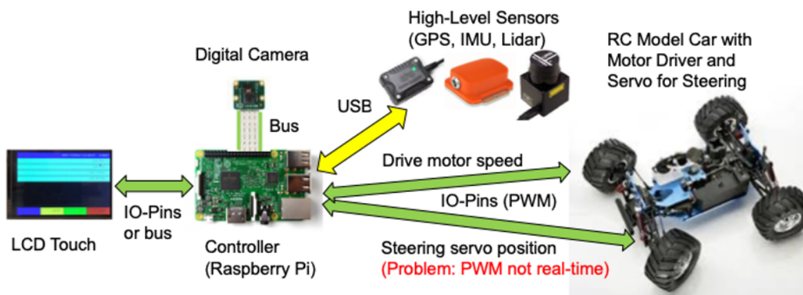
Figure 1.15: Robot system structure without I/O controller board
