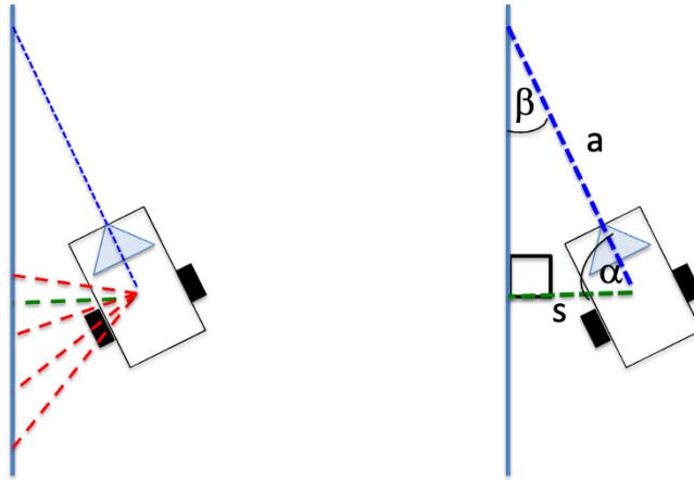
Figure 9.7: Lidar measures left and front of robot (left) and angle calculation from Lidar distances (right)
