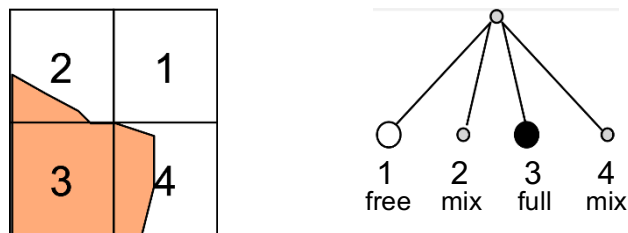
Figure 10.4: Quadtree step 1: four quadrants
