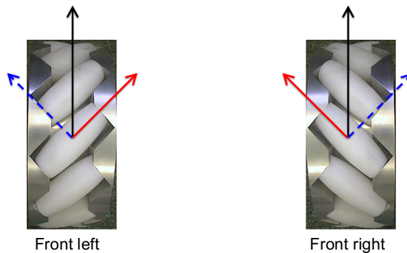
Figure 7.4: Forces on front-left and front-right Mecanum wheels
