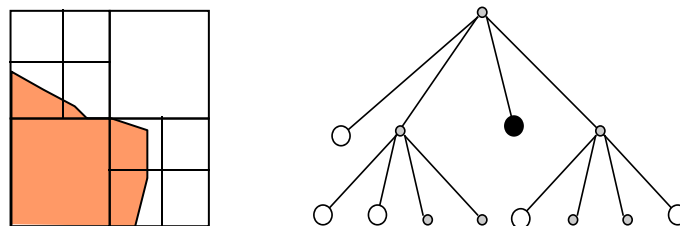
Figure 10.5: Quadtree step 2: further subdivision
