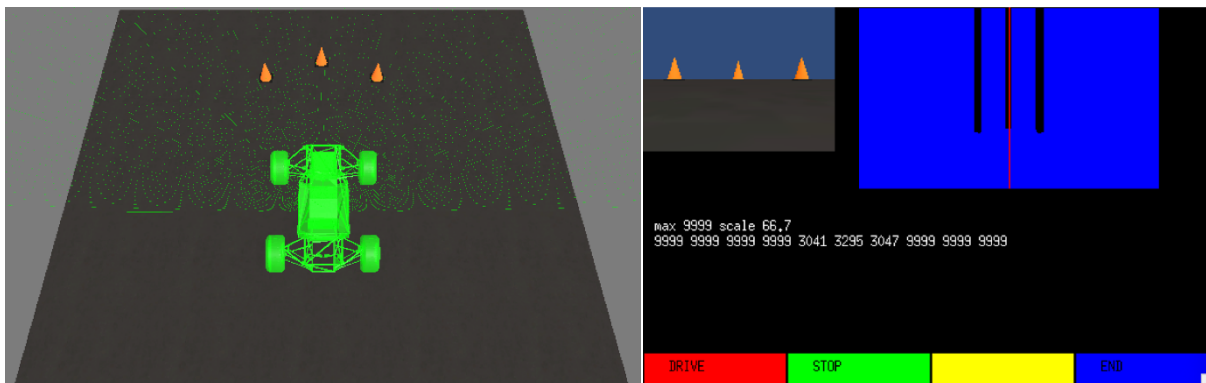
Figure 14.5: Testbed setup for cone detection using a Lidar
