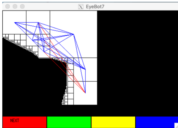
Figure 10.11: Quadtree decomposition with non-intersecting paths
