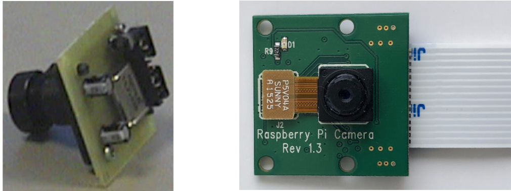
Figure 1.8: EyeCam M4 (left) and Raspberry Pi camera (right)
