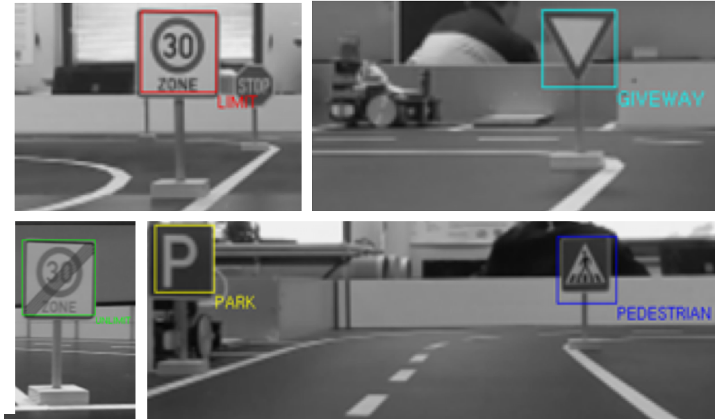
Figure 13.7: Traffic sign recognition in driving sequence
