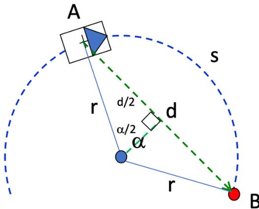
Figure 3.7: Driving arc calculation
