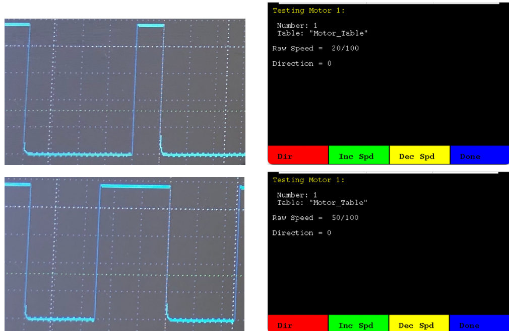
Figure 1.2: Motor output from pulse width modulation at 20% and 50%
