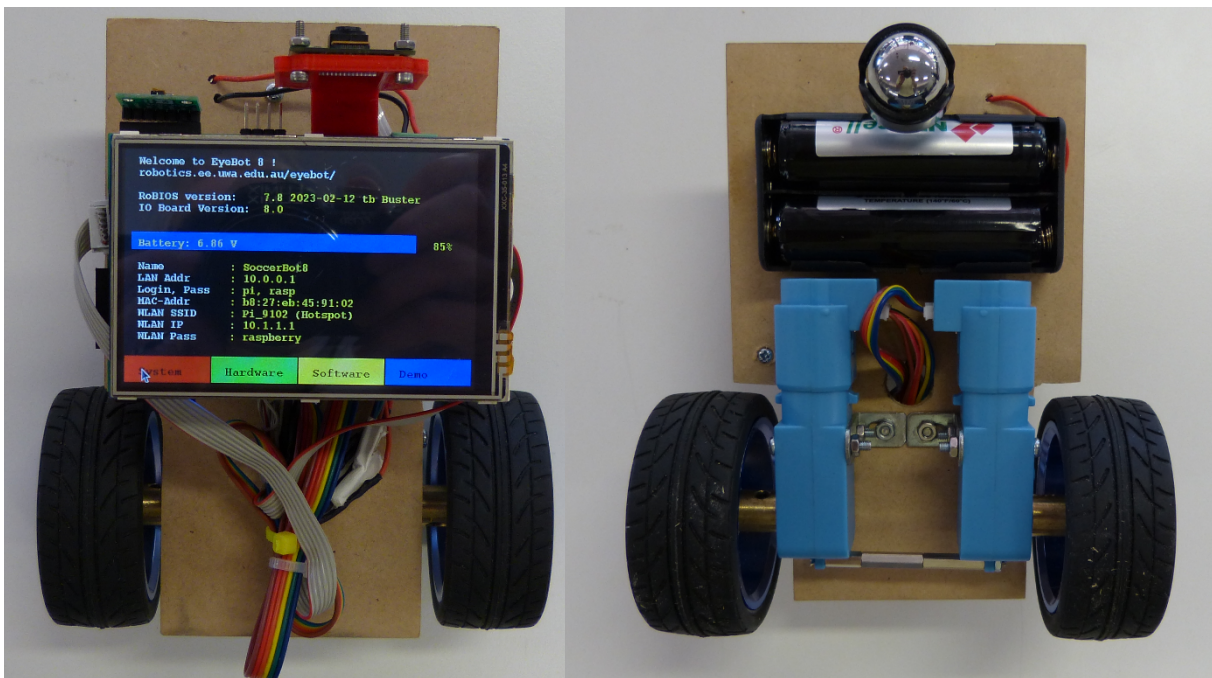
Figure 1.12: Simple robot design top and bottom
