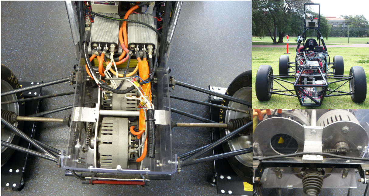
Figure 14.1: Vehicle chassis and dual motor drive system
