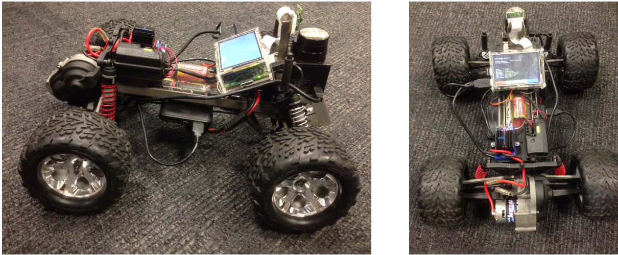
Figure 7.1: Model car with embedded controller, camera and Lidar
