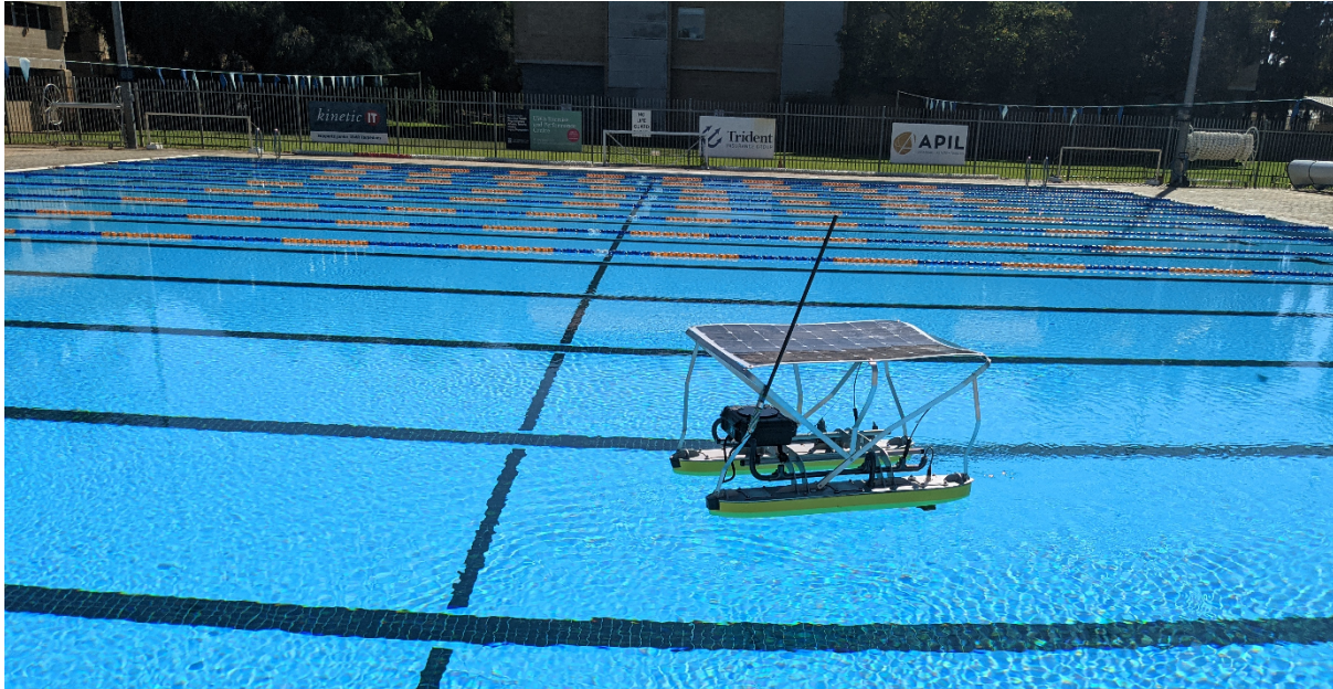
Figure 8.2: Autonomous Solar Boat training in the UWA pool
