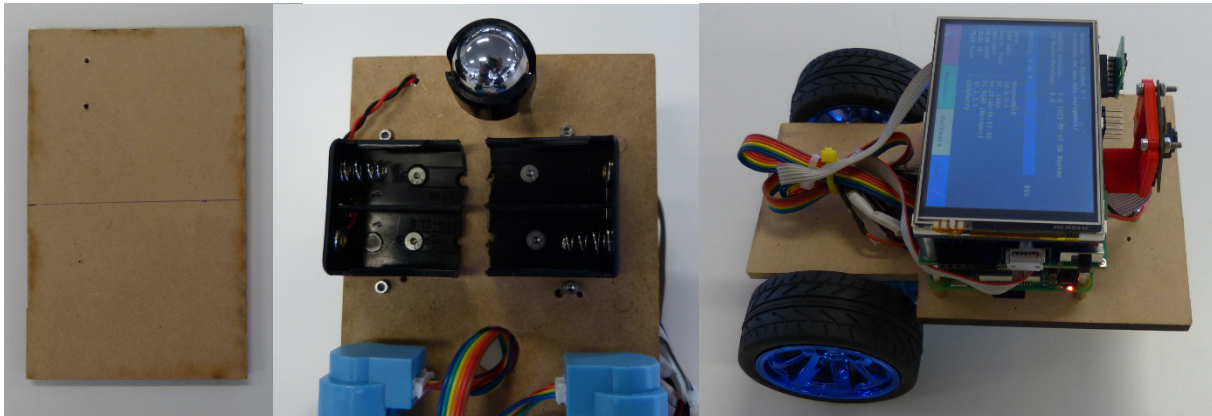
Figure 1.11: From empty plate to finished robot
