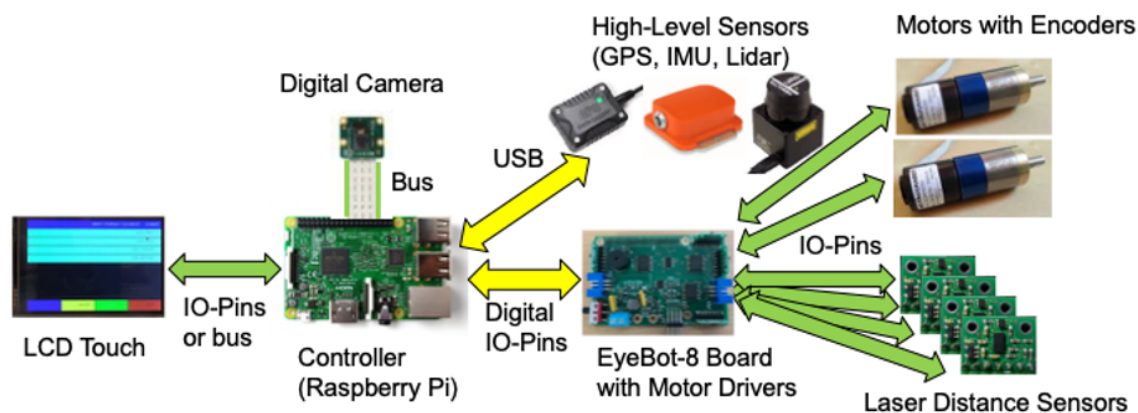
Figure 1.14: Robot system structure with I/O controller board
